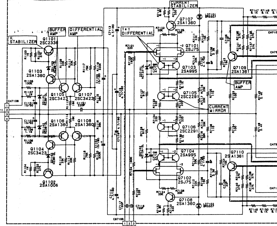
DRIVER P. C. Board
